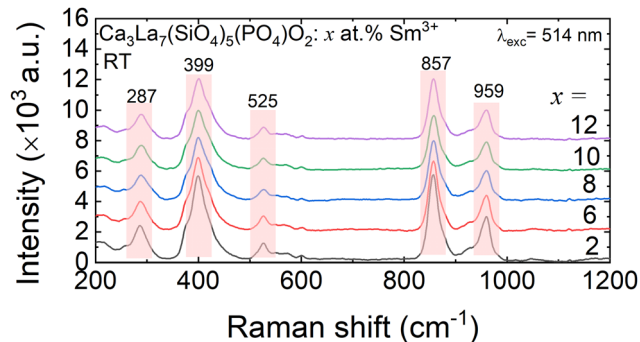
Fig. 6 Raman scattering spectra for \text{Ca}_3\text{La}_7(\text{PO}_4)_5(\text{SiO}_4)\text{O}_2:x \text{ at}\% \text{Sm}^{3+} ( x = 2, 6, 8, 10 and 12 ).
