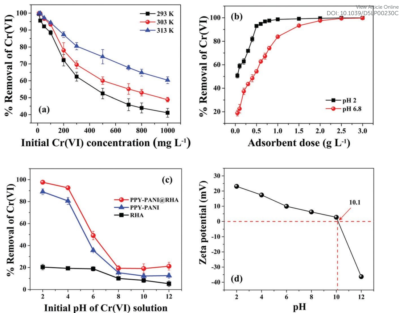
Figure 25 (a) Effect of initial concentration of Cr(VI) at a different temperature (PPY PANI@RHA dose: 0.8 \text{ g L}^{-1} ; contact time: 300 min; agitation speed: 200 rpm; pH~2), (b) Effect of adsorbent dose at pH 2 and without pH (~6.8) adjustment (initial Cr(VI) concentration: 50 \text{ mg L}^{-1} ; contact time: 300 min; agitation speed: 200 rpm; temperature: 303 K), (c) Effect of initial solution pH on % removal of Cr(VI) by PPY-PANI@RHA, PPY-PANI and RHA adsorbents (Initial Cr(VI) concentration: 50 \text{ mg L}^{-1} ; contact time: 300 min; agitation speed: 200 rpm; temperature: 303 K), and (d) Variation of zeta potential of PPY-PANI@RHA at different pH. 448 Reproduced with permission from RSC.
