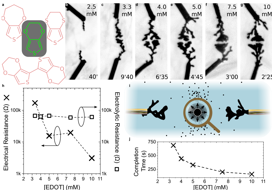
Figure 6: Influence of the Concentration of EDOT on CPD Morphogenesis | a , EDOT as a poorly but yet significantly more water soluble monomer than other structurally similar derivatives, such as 3,4-propylenedioxythiophene, 3,4-ethylenedithiathophene or the dimer of EDOT, which are insoluble in water. b-g , Optical pictures of CPD growths (4 V p , 0 V off , 80 Hz, 50% dc , 10 mM BQ and 1 mM NaPSS in water) with different molar concentrations of EDOT (values displayed at the top of each picture). Each image was taken a few seconds before CPDs merged (applied-voltage duration displayed at the bottom of each picture). h , Dependence of the electrical resistance (through each CPD displayed in Fig.6.b-g after they merged) and the electrolytic resistance (evaluated by impedancemetry at 10 kHz with a silver wire) on the concentration of EDOT in the growth media. i , Schematic of a growth mechanism limited by the concentration of EDOT where the kinetics of the reaction are influenced by the particle density and size distribution in the medium. j , Dependence of the completion time of each CPD displayed in Fig.6.b-g on the concentration of EDOT in the growth media.
