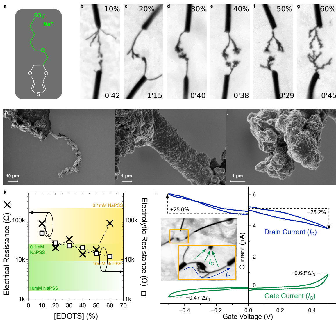
Figure 8: Influence of EDOT-S as an Electroactive Conjugated Polyelectrolyte Precursor on CPD Morphogenesis in Water | a , Chemical structure of EDOT-S. b-g , Optical pictures of CPD growths (4 V p , 0 V off , 80 Hz, 50% dc , 10 mM of total monomer content and 10 mM BQ in water) with different molar ratios of EDOT-S copolymerized with EDOT (values displayed at the top of each picture). Each image was taken a few seconds before CPDs merge (applied-voltage duration displayed at the bottom of each picture). h-j , SEM images of a CPD growth in the same conditions as displayed in Fig.8.f. k , Dependence of the electrical resistance (through each CPD displayed in Fig.8.b-g after they merge) and the electrolytic resistance (evaluated by electrochemical impedance spectroscopy at 10 kHz with a silver wire) on the molar ratio of EDOT-S copolymerized with EDOT. l , Transfer characteristic of the CPDs displayed in Fig.8.b-g in a merged state, using a silver wire as a gate electrode (as displayed in the inset).
