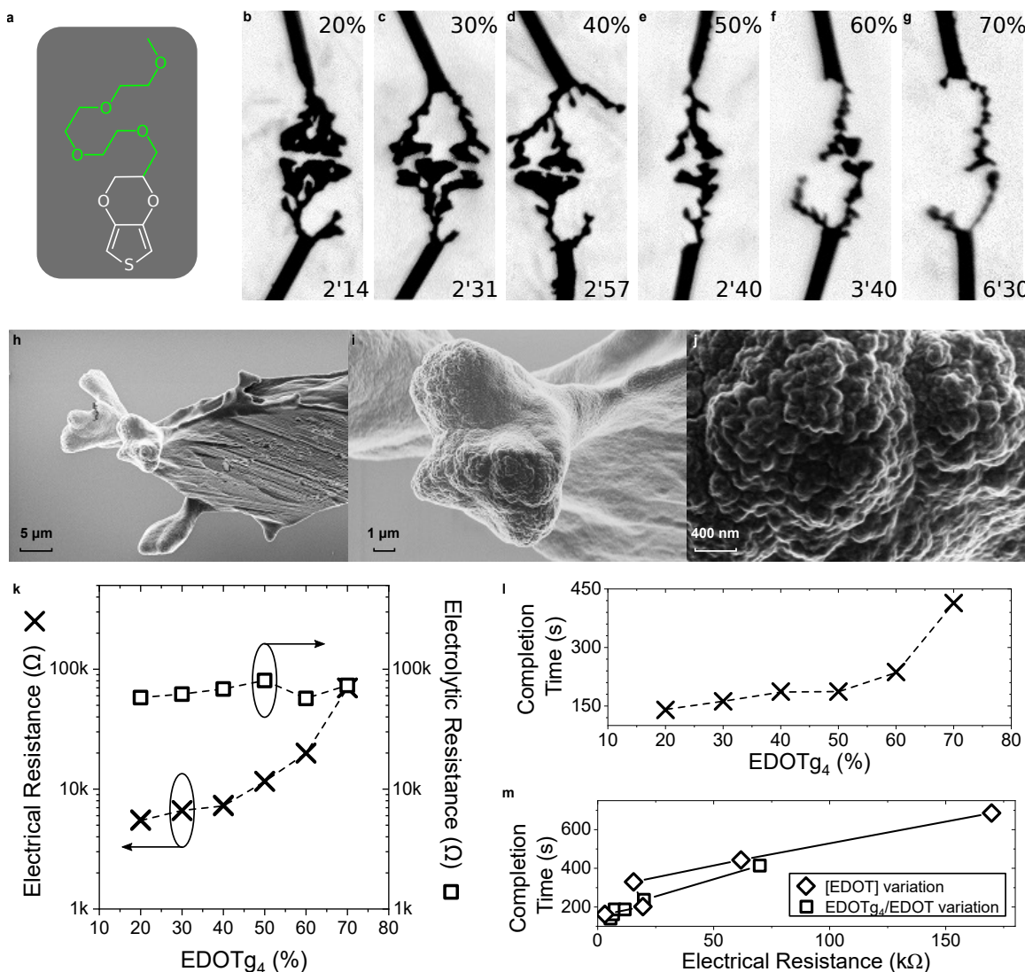
Figure 7: Influence of an Increased Monomer Hydrophilicity with EDOTg 4 on CDP Morphogenesis in water | a , Chemical structure of EDOTg 4 , as a structural analogue of EDOT with a hydrophilic side chain, synthesized as already reported by Ghazal et al. 60 b-g , Optical pictures of CPD growths (4 V p , 0 V off , 80 Hz, 50% dc , 10 mM of total monomer content, 10 mM BQ and 1 mM NaPSS in water) with different molar ratios of EDOTg 4 copolymerized with EDOT (values displayed at the top of each picture). Each image was taken a few seconds before CPDs merged (applied-voltage duration displayed at the bottom of each picture). h-j , SEM images of a CPD growth in the same conditions as displayed in Fig. 7.g. k , Dependence of the electrical resistance (through each CPD displayed in Fig. 7.b-g after they merged) and the electrolytic resistance (evaluated by impedancemetry at 10 kHz with a silver wire) on the molar ratio of EDOTg 4 copolymerized with EDOT. l , Dependence of the completion time on the molar ratio of EDOTg 4 copolymerized with EDOT. m , Comparison between the influence of EDOT dilution caused by EDOTg 4 substitution at 10 mM total content of monomers on growth latency and electrical resistance, and the results obtained in Fig. 6 for EDOT variation only.
