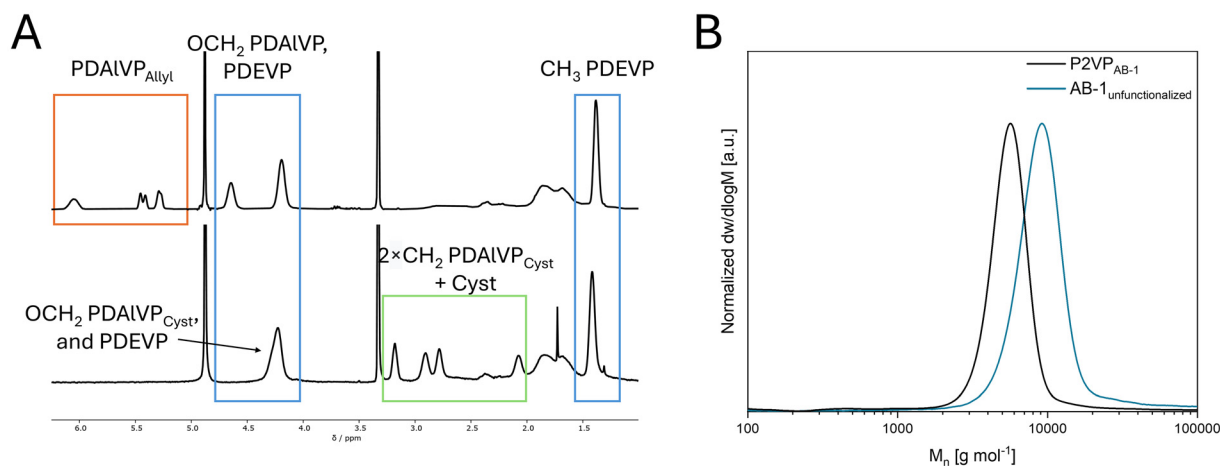
Fig. 1 (A) ^1\text{H-NMR} spectra showing successful and quantitative thiol-ene functionalization of \text{ABB}'\text{-}2_{\text{Allyl}} (A, top), resulting in \text{ABB}'\text{-}2_{\text{Cyst}} (A, bottom). Blue: Aliphatic side-chain protons of phosphorus-containing monomer units. Orange: Allylic protons of PDAIVP. Green: \text{CH}_2 protons of the former allyl group and cysteamine protons incorporated into \text{ABB}'\text{-}2_{\text{Cyst}} (B) SEC traces of block A (black) and AB (blue) of block copolymer AB-1 showing successful block copolymer formation indicated by a shift of the signal towards higher molar masses.
