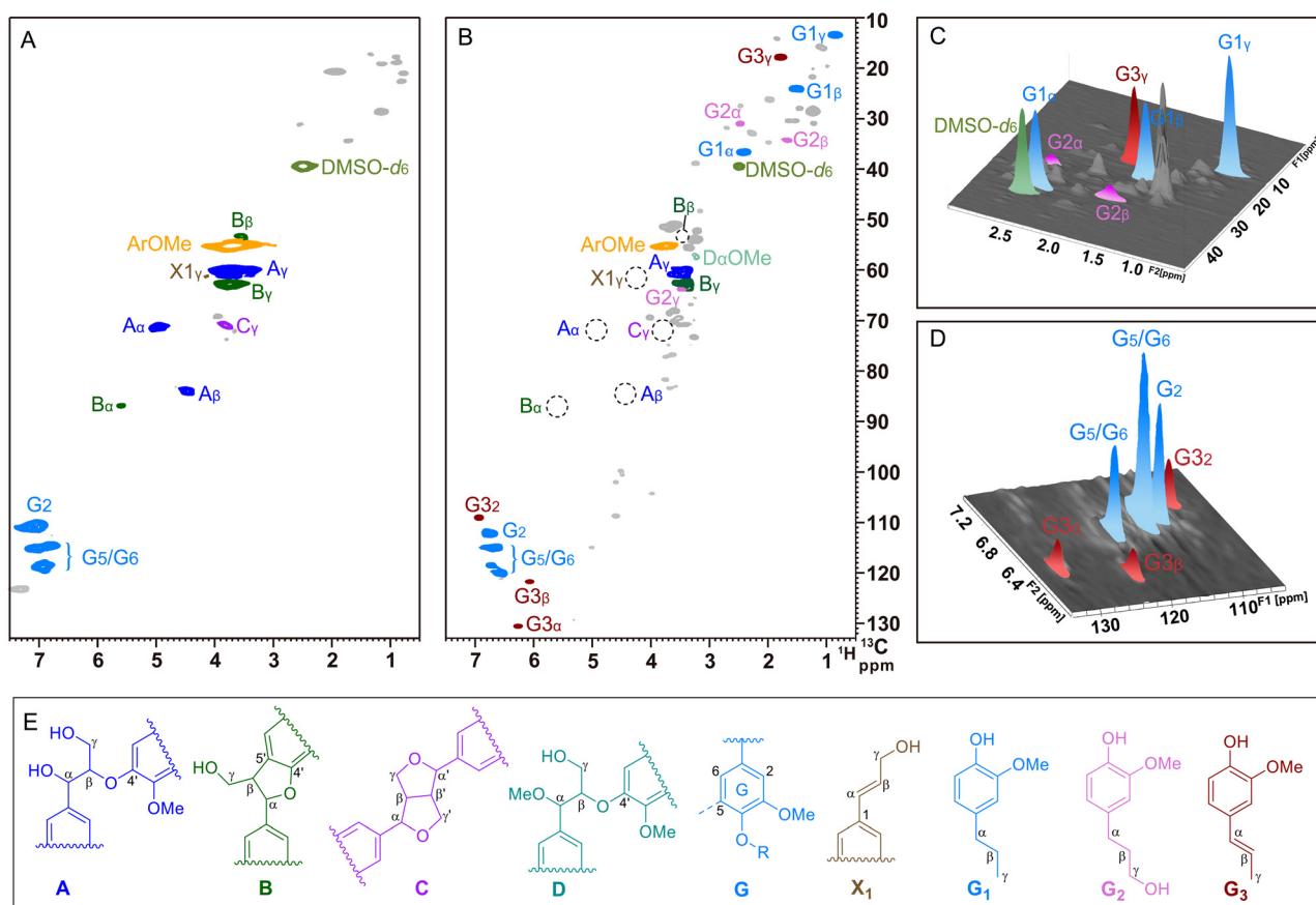
Fig. 6 Characterization of pine lignin and oily products. (A) 2D HSQC NMR spectrum of double enzymatic lignin (DEL) isolated from pine wood (dissolved in DMSO- d_6 ). (B) 2D HSQC NMR spectrum of the oily product from the Pd-Zn@CN reaction (dissolved in DMSO- d_6 ). (C and D) 3D version of the HSQC end-chain and aromatic regions. (E) Main structures presented in the 2D HSQC NMR spectra: (A) \beta -O-4' alkyl-aryl ether, (B) \beta -5' phenylcoumaran, (C) \beta - \beta' resinol, (D) \alpha -OH with methylated \beta -O-4' alkyl-aryl ether, (G) guaiacyl units, (X1) cinnamyl alcohol end-groups, (G1) dihydroeugenol, (G2) dihydroconiferyl alcohol, and (G3) isoeugenol.
