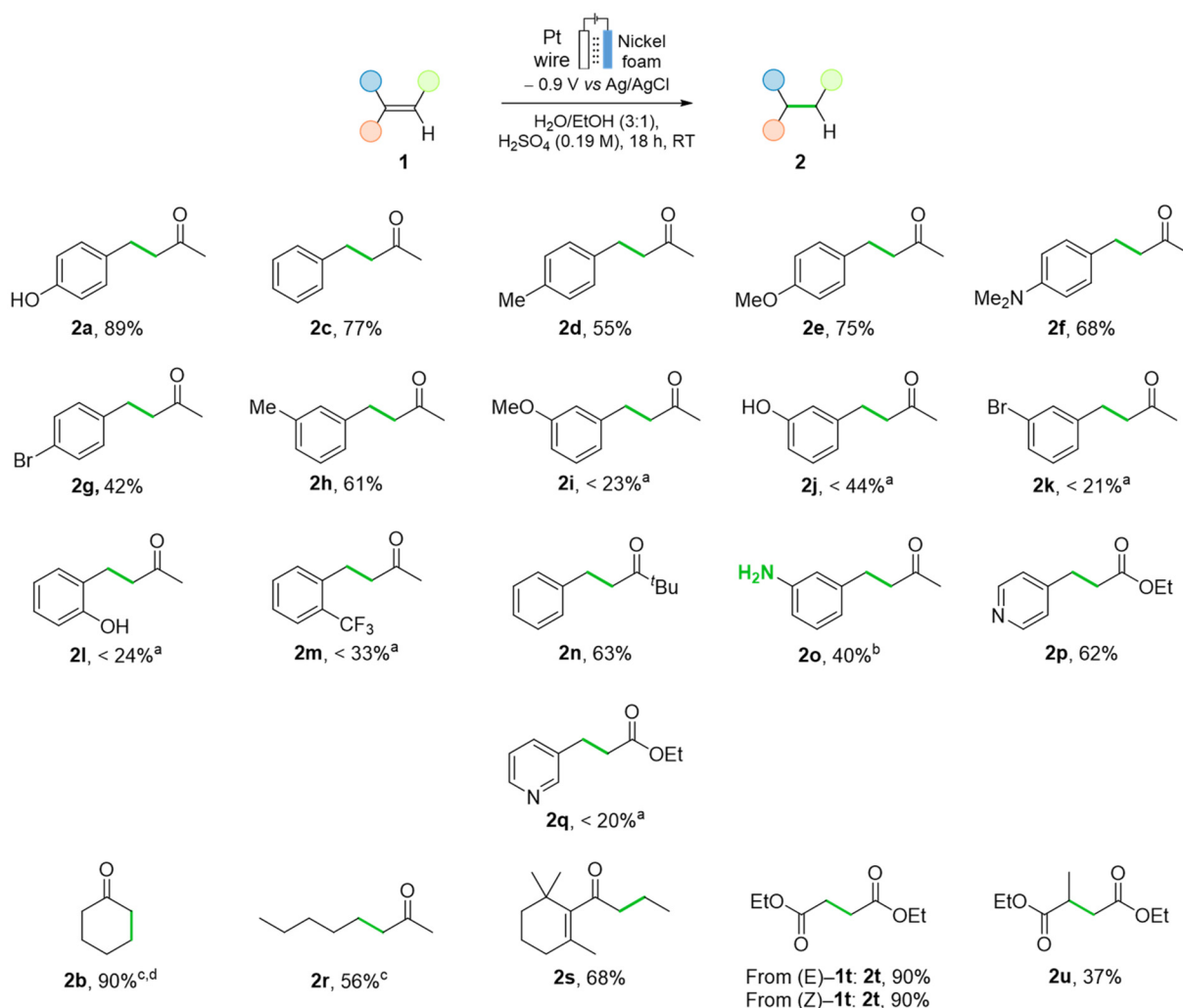
Fig. 8 Substrate scope and limitations. 1 (0.4 mmol, 0.016 M). a Yields were determined by ^1\text{H} NMR spectroscopy using an internal standard. b \text{H}_2\text{SO}_4 concentration was 0.38 M. c Yields were determined by GC-FID using a calibration curve. d 5 h.
