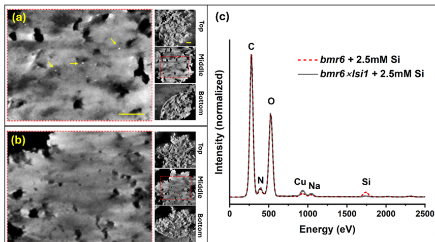
Fig. 10 Electron tomography of agglomerates of lignin extracted from bmr6 and bmr6 \times lsi1 plants, exposed to silicic acid at a concentration of 2.5 mM. (a) Thick virtual section reconstructed from the mid-plane of the bmr6 specimen; note the dense nanoparticles indicated by yellow arrows, which we identify as silica deposits due to the strong electron scattering. Insets to the right show the top, middle, and bottom sections to indicate the texture of small, clustered particles of lignin at the top and bottom. The bright circular arc in the bottom section is the edge of a hole (2 \mu m diameter) in the specimen support film. (b) Virtual sections of the bmr6 \times lsi1 specimen, organized as above. Bright nanoparticles were not observed. Scale bar in panel (a) is 200 nm, common to (a) and (b). Scale bar in the top inset is 200 nm, common to all insets. (c) EDX spectra recorded from the same grids, showing higher concentration of Si in the lignin extracted from the bmr6 plant than the bmr6 \times lsi1 plant.
