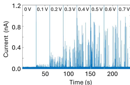
Fig. 6 Nanoimpact measurements of a solution of 0.04 \text{ mg mL}^{-1} 30 nm citrate Ag NPs dissolved in 20 mM KCl using a Pt ultramicroelectrode (10 \mu\text{m} in diameter) with increasing applied potential (as labelled). Reference electrode: Ag/AgCl frit filled with 20 mM KCl. Measurements performed with the Elements SRL nanopore reader at a sampling frequency of 100 kHz.
