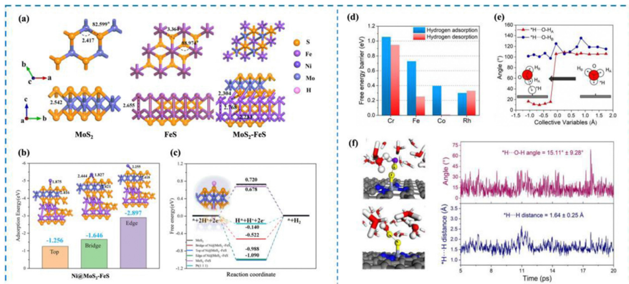
Fig. 4 Examples of theoretical computational methods to study HER mechanisms. (a) \text{MoS}_2 , FeS and \text{MoS}_2\text{-FeS} structure models. (b) Schematic diagram of adsorption energy of \text{Ni@MoS}_2\text{-FeS} single-atom catalysts at different sites. (c) \Delta G of electrocatalysts with different structures. (d) Hydrogen adsorption and hydrogen desorption on different catalysts. (e) Analysis of the angle between adsorbed hydrogen and the O–H bond of water. (f) AIMD simulation for illustration and analysis of the \text{H}\cdots\text{O}-\text{H} angle and \text{H}\cdots\text{H} distance. 118,119 This figure has been adapted from ref. 118 and 119 with permission from IOP Publishing and American Chemical Society, copyright IOP Publishing. Copyright©2023, American Chemical Society.
