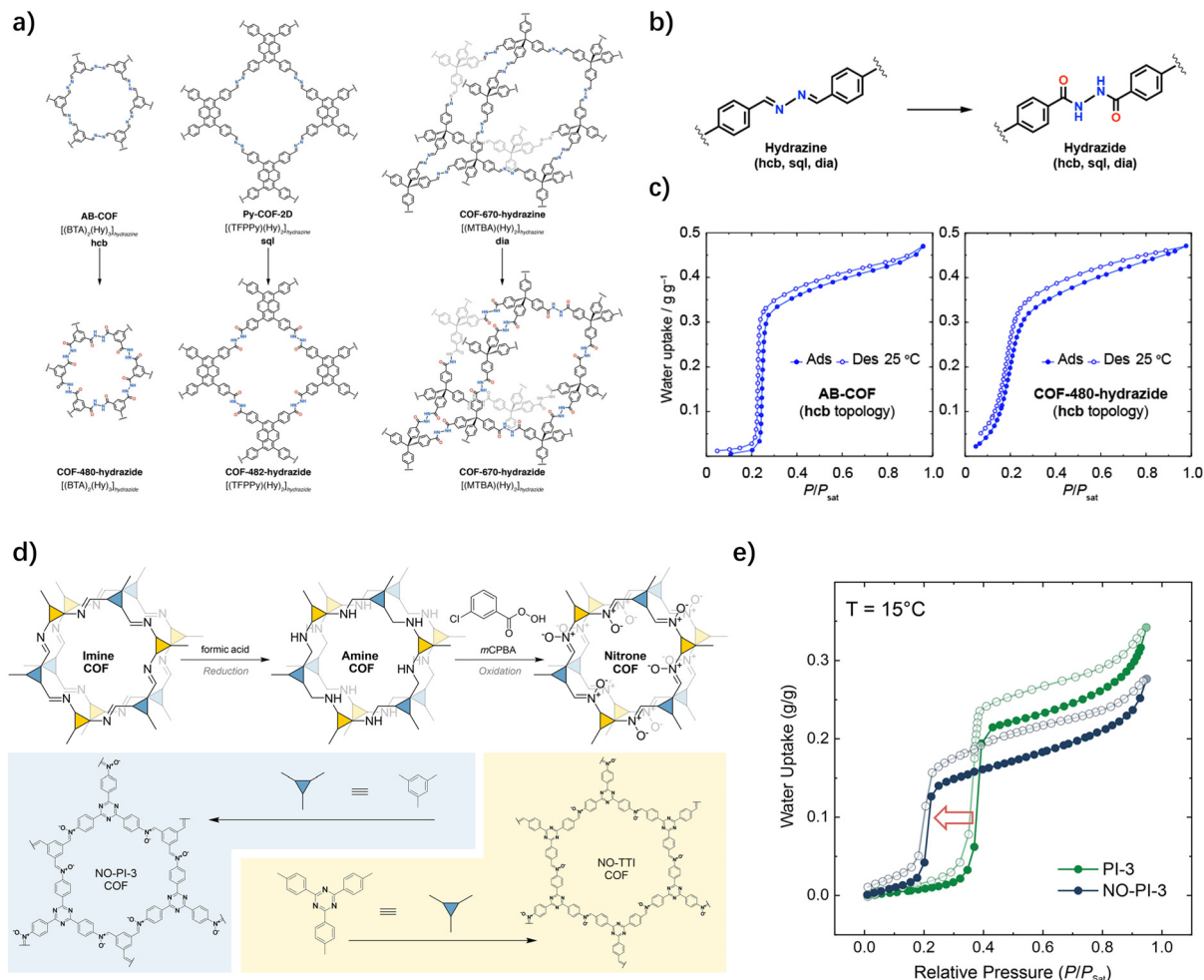
Fig. 7 (a) Overview of the synthesis of 2D hcb, 2D sq, and 3D dia hydrazide-linked COFs. (b) Synthetic scheme of transforming the hydrazine linkage into a hydrazide linkage. (c) Water isotherms of AB-COF and COF-480-hydrazide at 298 K. 28 (d) Synthetic scheme of transformation of the imine linkage into the nitron linkage. (e) Water isotherms of PI-3 COF and NO-PI-3 COF at 288 K. 29
