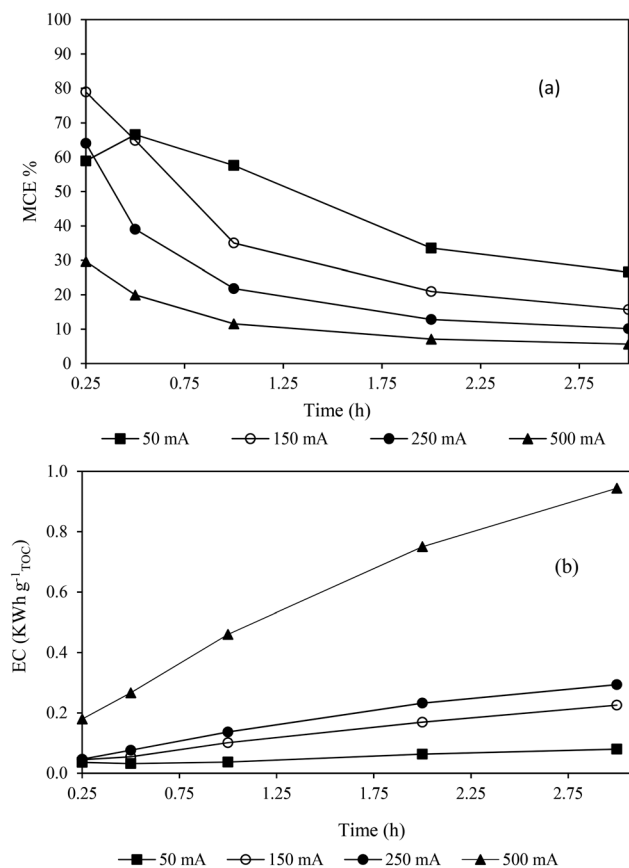
Fig. 3 Mineralization current efficiency (% MCE) (a) and energy consumption ( EC_{TOC} ) (b) as a function of electrolysis time of 50\ mg\ L^{-1} of miconazole corresponding to 25.95\ mg\ L^{-1} initial TOC by electro-Fenton under operating conditions of [Na_2SO_4] = 50 mM, Fe^{2+} = 0.2 mM and pH = 3.0.
