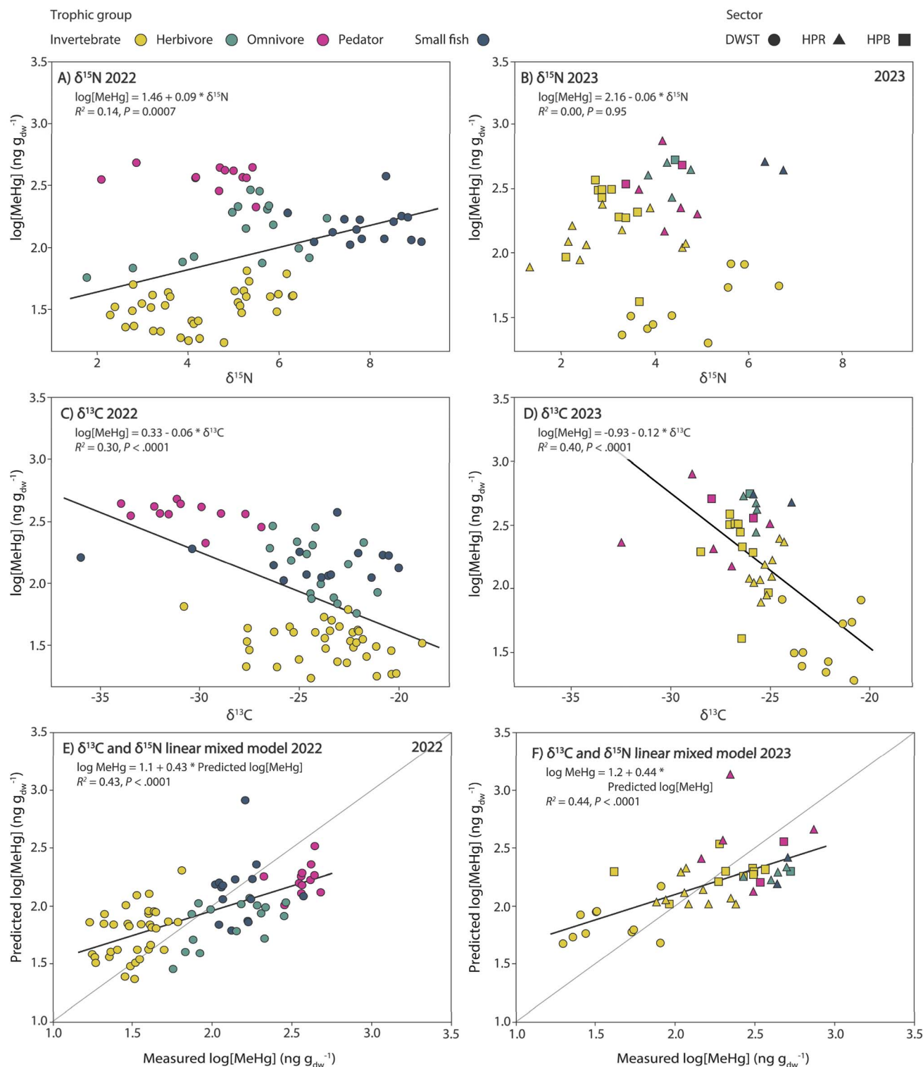
Fig. 5 Simple linear regressions of \log[\text{MeHg}] ( \text{ng g}_{\text{dwt}}^{-1} ) measured in biota plotted with \delta^{15}\text{N} (‰) (A and B) and \delta^{13}\text{C} (‰) (C and D)) in pre-flood conditions of 2022 (left panels) and three months post-flood in 2023 (right panels), and predicted \log[\text{MeHg}] from the \delta^{13}\text{C} and \delta^{15}\text{N} linear mixed model plotted with measured \log[\text{MeHg}] ( \text{ng g}_{\text{dwt}}^{-1} ) for 2022 (E) and 2023 (F). Trophic groups of invertebrates and small fishes are shown by the different colors while sampling sectors are highlighted by different shapes for the 2023 data only. A fit line is shown when the model is significant.
