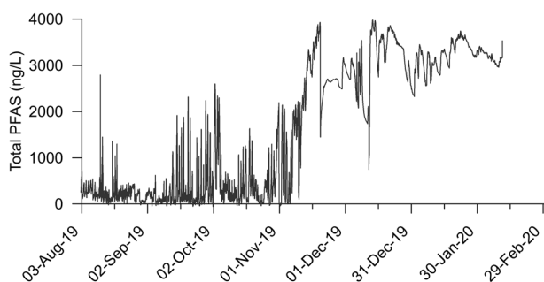
Fig. 5 Estimated concentration of total PFAS ( \sum SC + LC + USC) for epibenthic exposure within the HB pond plume footprint, based on continuous SpC measurements at ~1 cm above the pond sediments.
