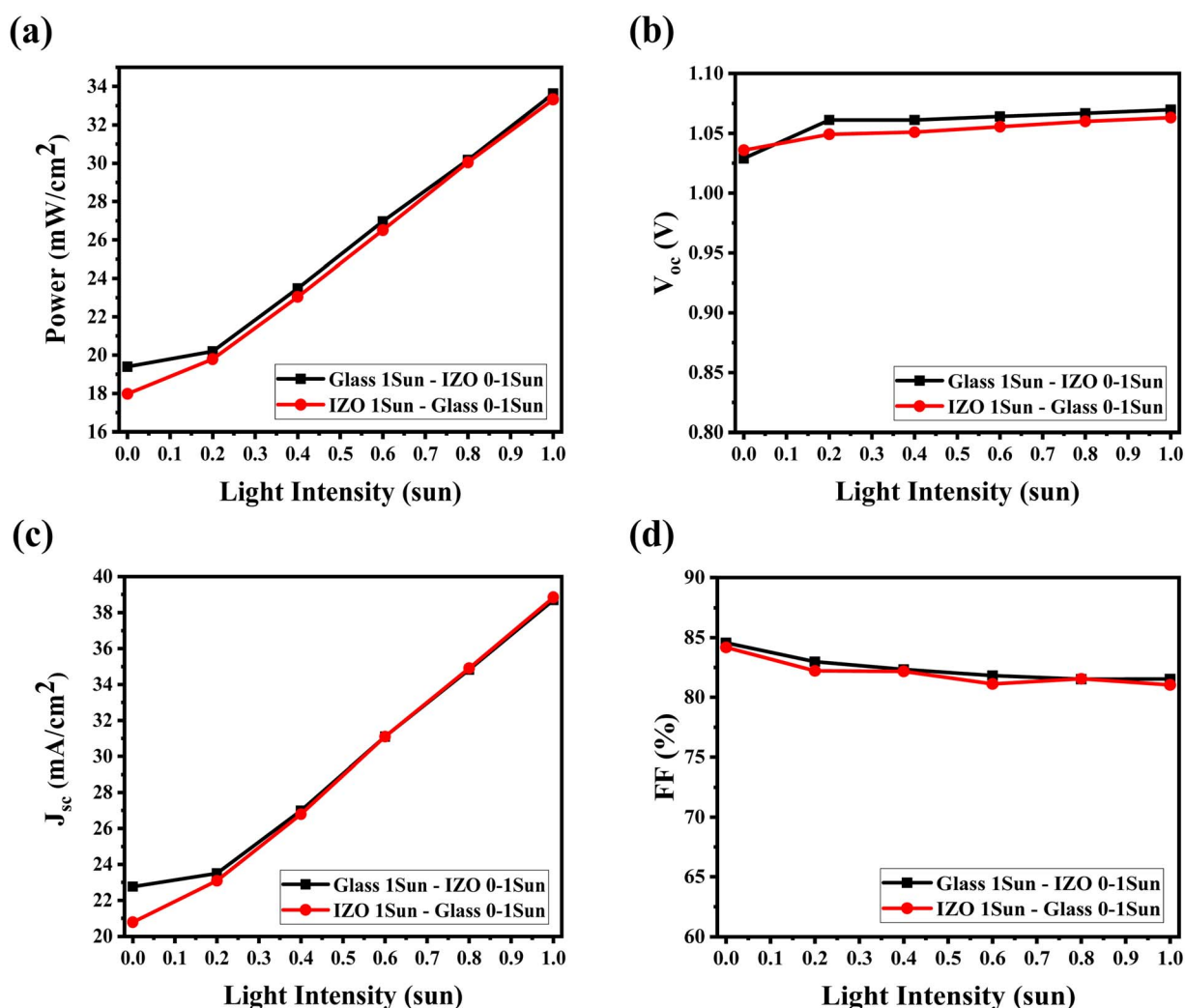
Fig. 16 (a) Power output and (b) V_{oc} (c) photocurrent and (d) FF of the MA free perovskite (FA 0.78 CS 0.22 Pb(I 0.85 Br 0.15 ) 3 ) bifacial illuminated device as a function of backside illumination intensities with fixed 1 sun intensity from glass (blackline) and IZO (red line) sides.
