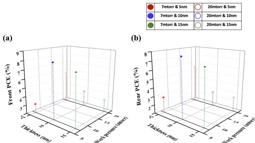
Fig. 5 For bifacial devices with sputtered buffer layers, measured under AM 1.5 G 1 sun illumination, the performance with different \text{SnO}_2 thicknesses and working pressures: (a) front-side efficiency and (b) rear-side efficiency.
