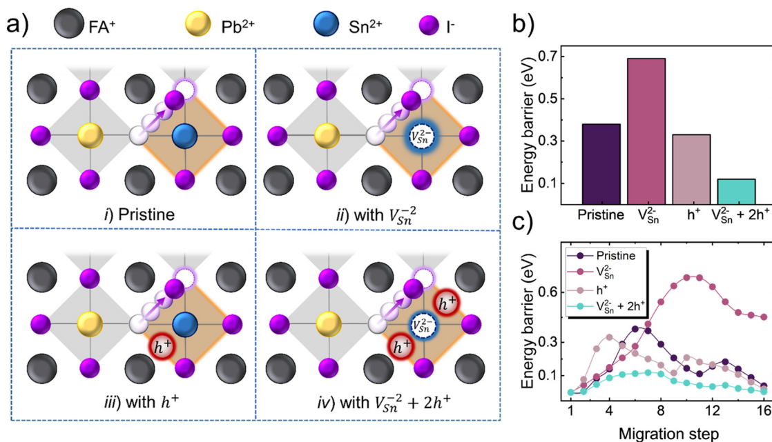
Fig. 4 (a) Theoretical model of the iodide migration pathway in a FAPb 0.5 Sn 0.5 I 3 lattice under four scenarios: (i) V 1 + ( i.e. the pristine case), (ii) V 1 + and V Sn 2- , (iii) V 1 + and h + , and (iv) V 1 + , V Sn 2- , and 2h + . (b) The energy barriers for iodide migration of each proposed scenario. (c) Relative energy landscapes of the system during iodide migration, the x-axis represents the iodide migration step during its transition towards an adjacent V 1 + .
