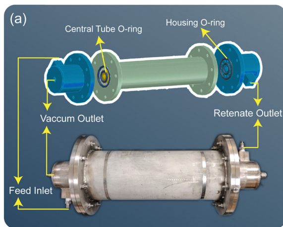
Fig. 16 Spiral wound module test rig for facilitated transport membrane assisted decarbonization; (a) schematic of the module's housing, (b) test setup (reproduced from ref. 197 with permission from Elsevier, copyright 2025).
