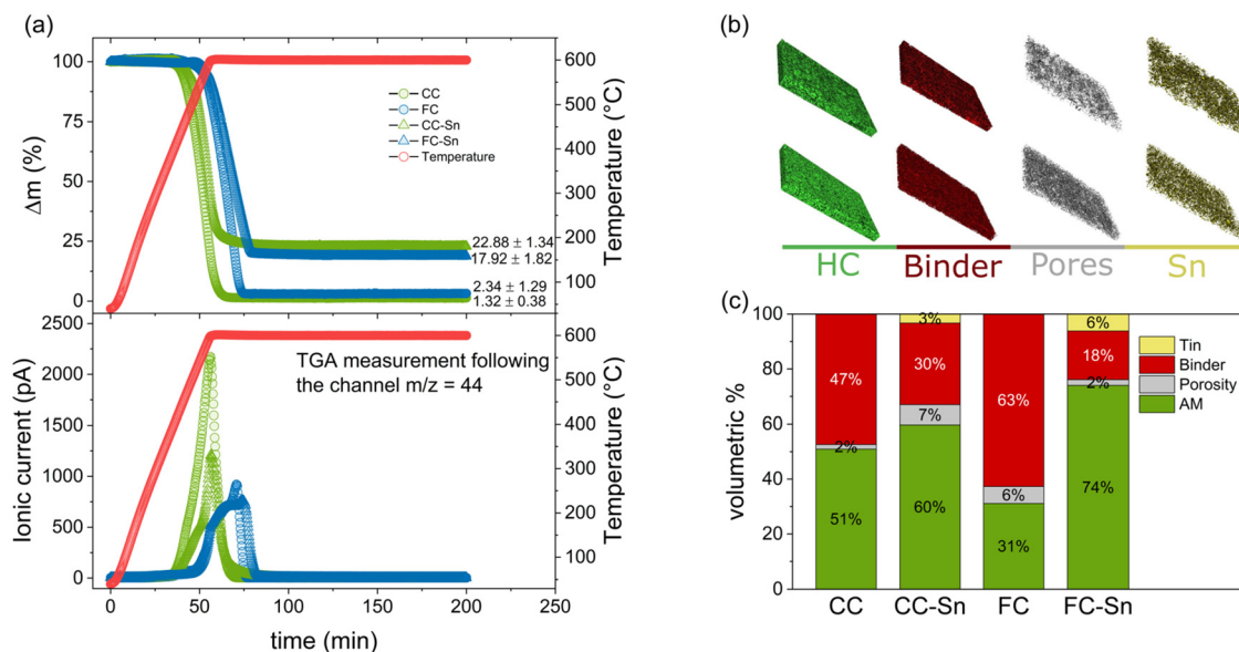
Fig. 3 (a) Residual mass of the HCs and composites after TGA-MS in air and relative ionic current given by CO 2 evolution. (b) 3D XRM reconstructions of the section of composite electrodes (CC-Sn on top and FC-Sn on the bottom). (c) Volumetric% of electrode components.
