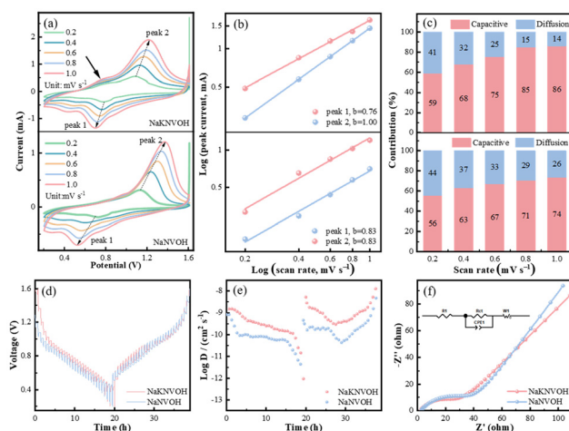
Fig. 4 Electrochemical kinetic mechanism of NaNVOH and NaKNVOH cathodes. (a) CV curves at different scan rates. (b) Relationship between peak currents and scan rates. (c) Pseudocapacitive contribution at various scan rates. (d) GITT curves and (e) calculated diffusion coefficients of Zn 2+ . (f) EIS spectra with fitted equivalent circuit diagrams.
