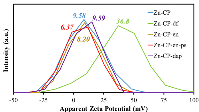
Fig. 11 Zeta potential curves of Zn-CP and its PSM derivatives.
