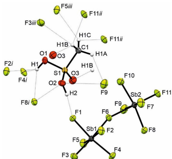
Fig. 6 Short contacts of the asymmetric unit of 3 (displacement ellipsoids with 50% probability). Symmetry codes: i = -x, 1/2 + y, 1/2 - z ; ii = -x, -y, -z ; iii = x, 1/2 - y, 1/2 + z .
