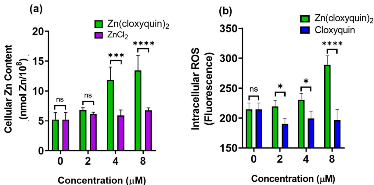
Fig. 3 The intracellular Zn concentration of MSSA bacteria treated with Zn(cloxyquin) 2 or ZnCl 2 (a), and the relative yield of intracellular ROS generation in MRSA a bacterial cells treated with Zn(cloxyquin) 2 or cloxyquin (b) (mean \pm s.d., n = 3 replicates; * p < 0.05 , *** p < 0.001 , **** p < 0.0001 and ns = not significant).
