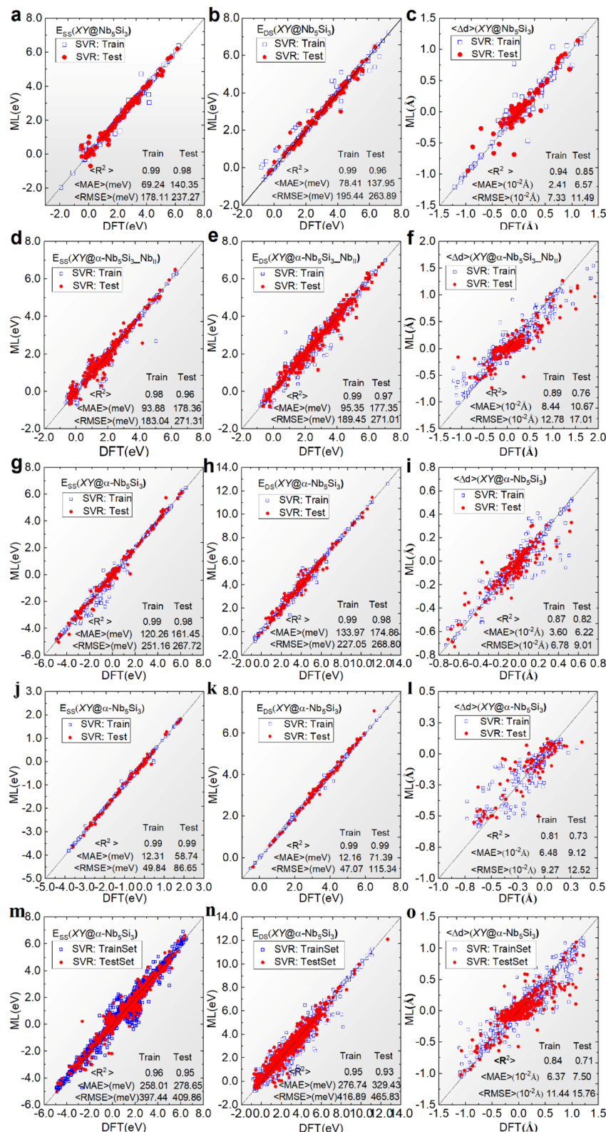
Fig. 4 E_{SS} , E_{DS} , and \langle \Delta d \rangle of the \alpha -Nb 5 Si 3 substitution systems at the four non-equivalent sites (a–c) Nb I , (d–f) Nb II , (g–i) Si I , (j–l) Si II , and (m–o) all sites predicted by the CE AET -SVR models compared with the DFT results.
