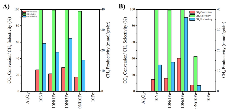
Fig. 6 CO 2 conversion and CH 4 selectivity during thermal-catalytic CO 2 methanation at 300 °C by 10Ni, 10Fe and 10NixFe (where x = 1, 3, 10) Al 2 O 3 -supported catalysts. Neat Al 2 O 3 is included as a control. Where: A) WI; B) DP.
