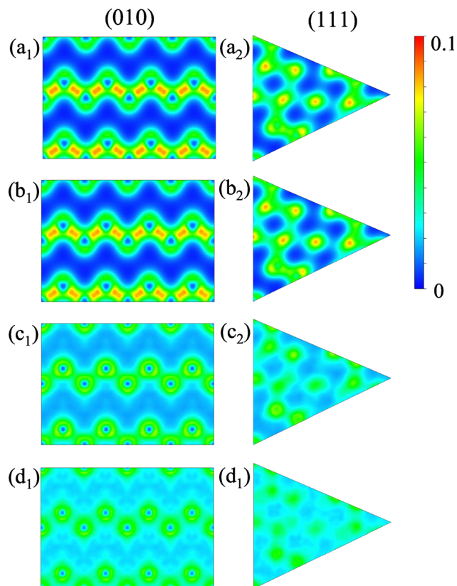
Fig. 8 Two-dimensional snapshots of the electron density distributions of the silicon crystal along the (010) ( a_1 )–( d_1 ) and (111) ( a_2 )–( d_2 ) planes after laser irradiation. Panels correspond to laser intensities: ( a_1 ) and ( a_2 ) I = 0 \text{ W cm}^{-2} , ( b_1 ) and ( b_2 ) I = 1 \times 10^{12} \text{ W cm}^{-2} , ( c_1 ) and ( c_2 ) I = 1 \times 10^{14} \text{ W cm}^{-2} , and ( d_1 ) and ( d_2 ) I = 1 \times 10^{15} \text{ W cm}^{-2} .
