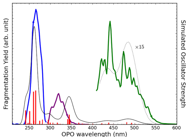
Fig. 3 Optical action (fragmentation) spectrum of [\text{Mo}_6\text{I}_{14}]^{2-} in the UV-visible range. The photo-fragmentation was recorded independently for three regions: <290 nm (blue), [290\text{--}390] nm (purple) and >410 nm (green). Laser irradiance and alignment conditions vary between regions so that their absolute intensities should not be compared. Thus, experimental data was scaled to ease the comparison with the simulated spectrum. Data were recorded with a 2 nm pitch. Circles on the experimental curves represent the position of the laser alignment for each spectral range. The simulated spectrum (thin black line) is calculated from 0.12 eV Gaussian convolution of the oscillator strength for each transition (red bars). A factor \times 15 is applied to simulated data in the visible range (dotted line).
