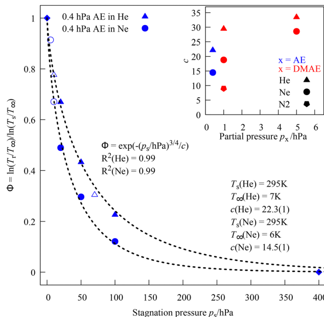
Fig. 3 Interpolation function \Phi(T_r) between stagnating and expanding AE at 0.4 hPa mixed with He and Ne up to 400 hPa stagnation pressure (diamonds). The smaller the fitted c parameter and the heavier the carrier gas, the faster the rotation cools with increasing stagnation pressure. Filled symbols are included in the fit, empty symbols are test data. The insert shows fitted c parameters as a function of partial pressure for different aminoalcohols and carrier gases. See ESI† for details.
