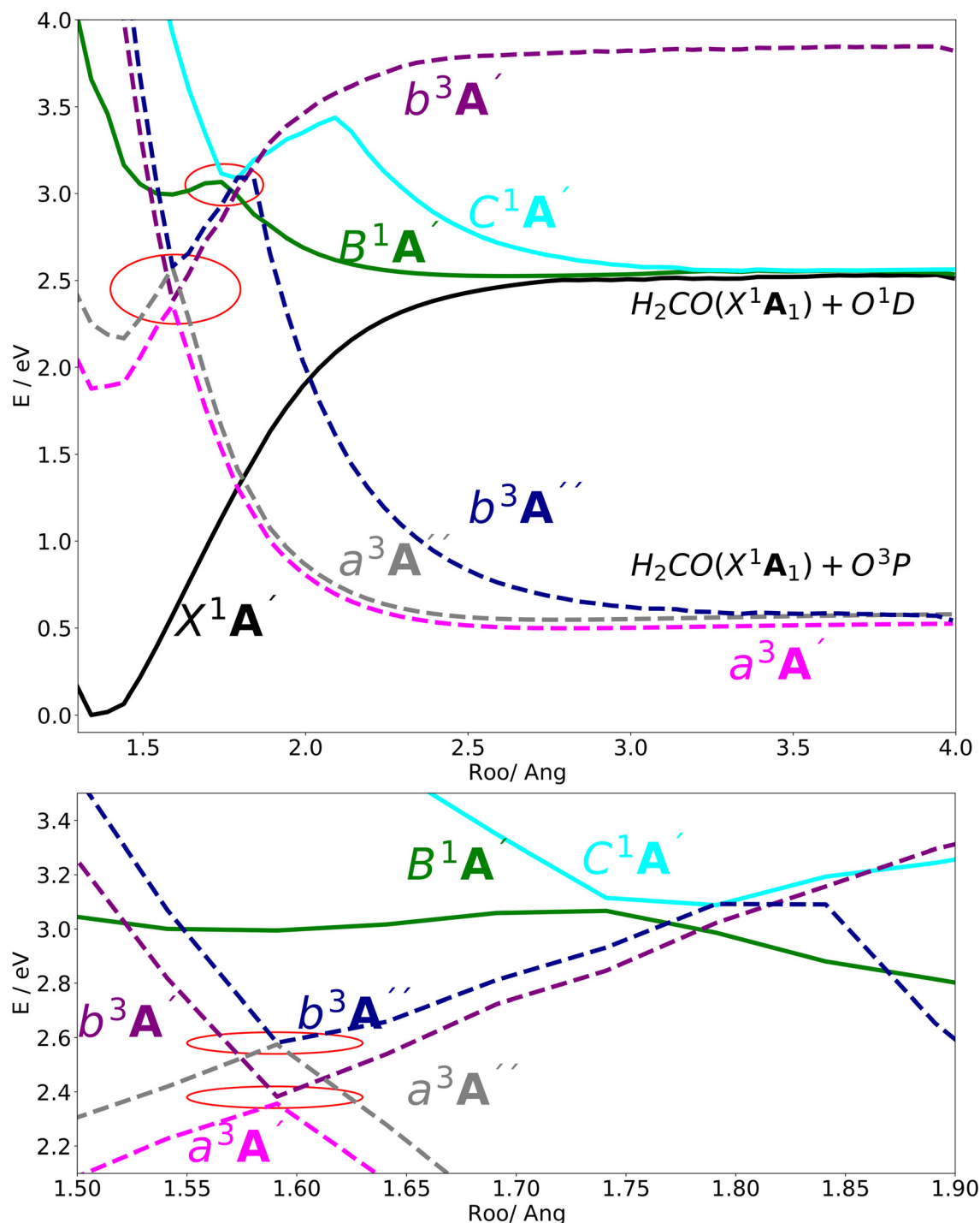
Fig. 19 (Upper) the adiabatic PE curves along the \text{O}-\text{O} stretching mode for the X^1A' , B^1A' , C^1A' , a^3A' , b^3A' , a^3A'' and b^3A'' states. (Lower) the adiabatic PE curves along \text{O}-\text{O} stretching mode, zooming in geometries in the range 1.55 < R_{\text{OO}} < 1.80 (indicated by red circles in the upper panel). The bonding angle \theta_{\text{COO}} and the stretching mode R_{\text{CO}} are fixed at the equilibrium structure values 117.905^\circ and 1.27 , respectively.
