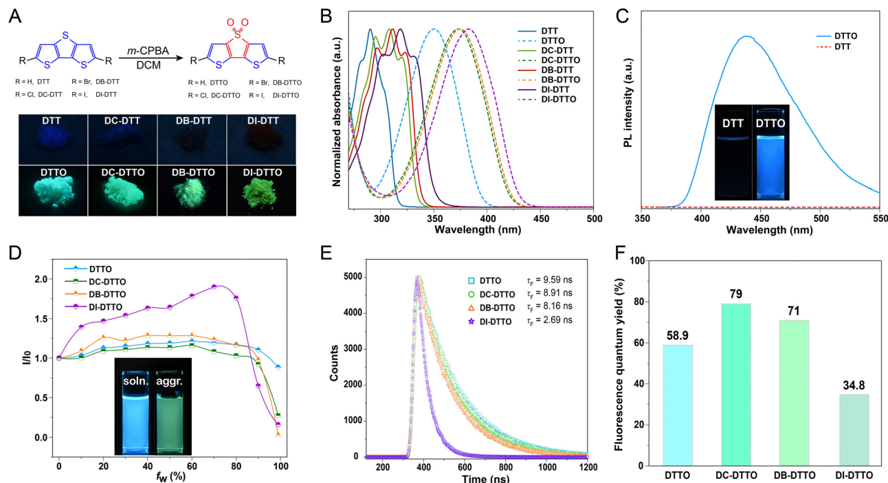
Fig. 2 (A) Synthetic route and molecular structures of DTTs and DTTOs. (B) UV-vis spectra of DTTs and DTTOs. (C) PL spectra of DTT and DTTO in THF solution. (D) Plots between the ratio of I/I_0 and water fraction in H_2O/THF mixtures; I_0 and I are the maximum PL intensity of DTTOs in pure THF and in H_2O/THF mixtures (concentration: 1 \times 10^{-5} \text{ mol L}^{-1} ), respectively; inset: fluorescence photograph of DI-DTTO in pure THF and in 99% H_2O/THF mixtures taken under 365 nm UV irradiation. (E) Fluorescence lifetimes, and (F) fluorescence quantum yields of DTTOs in THF solutions.
