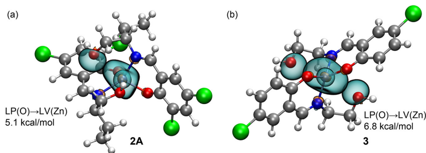
Fig. 21 Plots of the NBOs involved in the LP(O) \rightarrow LV(Zn) charge transfer and the second order perturbation energies in complexes 2A (a) and 3 (b). In complex 3 , the structure has been simplified for clarity, showing only the fragment comprising the Zn 2 coordination sphere.
