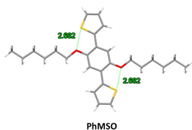
Fig. 9 X-ray structure of PhMSO .
