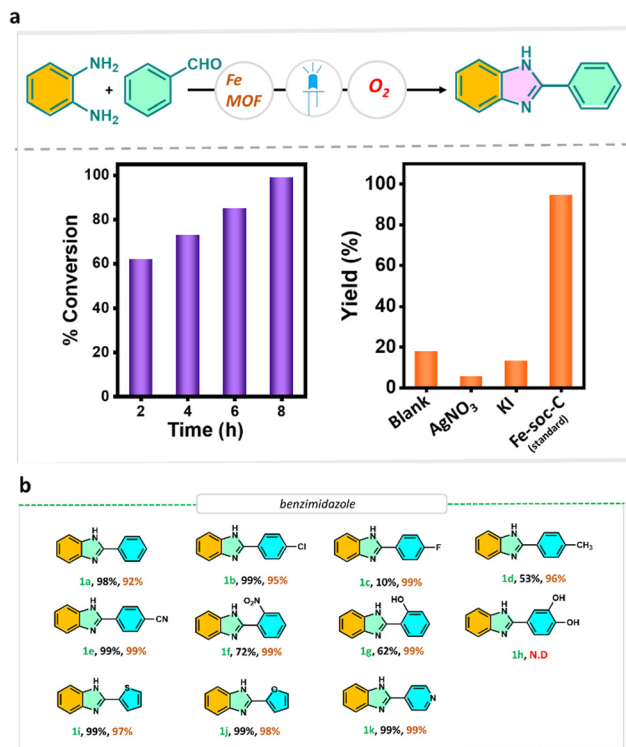
Fig. 3 (a) Photocatalytic activity of Fe-soc-C for benzimidazole synthesis and optimization study, (b) substrate scope. Conversions were calculated using GC-MS analysis (conversions were indicated in black and selectivity was indicated in red).
