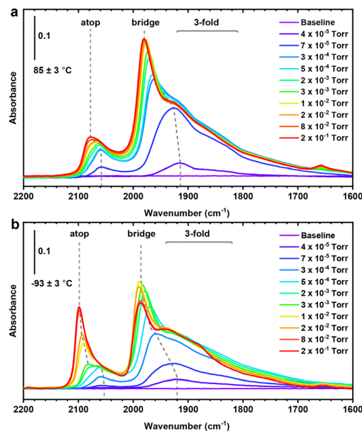
Fig. 2 DRIFT spectra showing CO adsorption over a 5% Pd/Al 2 O 3 catalyst as a function of CO partial pressure in the DRIFTS cell at (a) 85 °C, and (b) -93 °C.
