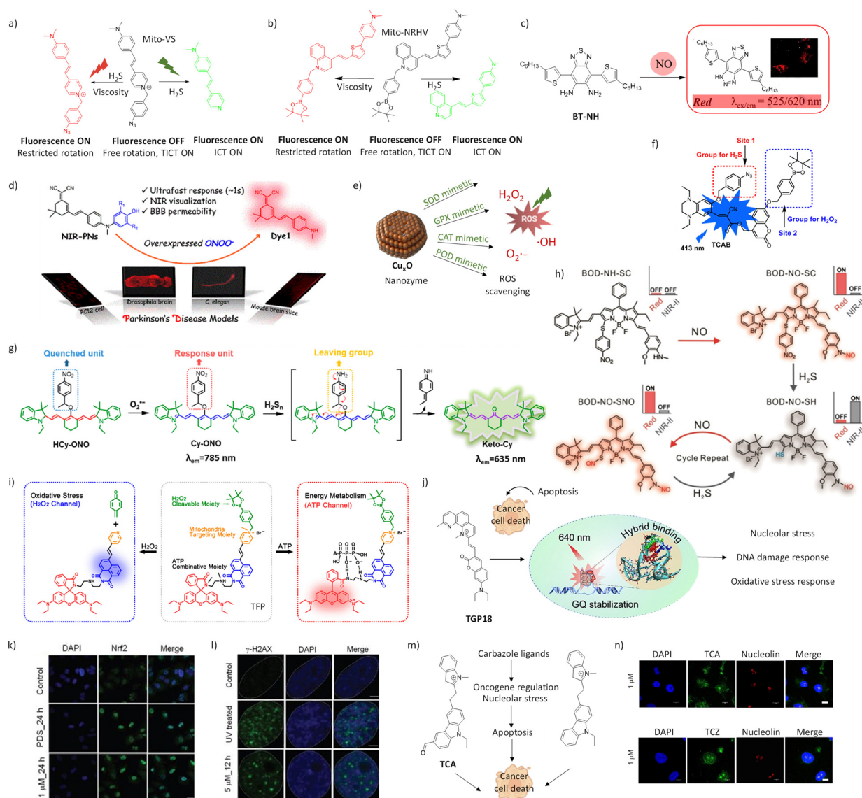
Fig. 7 (a) Design of dual-responsive fluorescent probe Mito-VS for detection of viscosity and H 2 S. Reproduced with permission from ref. 80. Copyright 2018 American Chemical Society. (b) Design of dual-responsive fluorescent probe Mito-NRHV for detection of viscosity and H 2 S. Reproduced with permission from ref. 81. Copyright 2020 Royal Society of Chemistry. (c) Design of BT-NH for the specific detection of NO within the brains of PD animal models. Reproduced with permission from ref. 82. Copyright 2019 Elsevier. (d) Design of NIR-PNs , a class of near-infrared probes for ultra-fast and highly selective detection of ONOO - across various PD animal models. Reproduced with permission from ref. 83. Copyright 2020 American Chemical Society. (e) Design of Cu 2 O nanoclusters . Reproduced with permission from ref. 76. Copyright 2019 American Chemical Society. (f) Design strategy of TCAB for the precise detection of H 2 S and H 2 O 2 simultaneously. Reproduced with permission from ref. 86. Copyright 2020 American Chemical Society. (g) Design strategy for HCy-ONO that offers dual turn-on fluorescence responses for H 2 Sn and O 2 •- in separate windows. Reproduced with permission from ref. 87. Copyright 2019 American Chemical Society. (h) Design strategy for BOD-NH-SC , an (ESIPT)-based 'AND' logic system probe, tailored for imaging thiols and ONOO - in cellular environments. Reproduced with permission from ref. 88. Copyright 2021 Wiley. (i) Design strategy for TFP for simultaneous determination of mitochondrial H 2 O 2 and ATP changes in two well-separated fluorescence channels. Reproduced with permission from ref. 89. Copyright 2020 American Chemical Society. (j) Structure of TGP18 and schematic showing its binding to GQ and subsequent cancer cell death. (k) Immunofluorescence images of A549 cells showing nuclear translocation of Nrf2 (green) upon treatment with TGP18. Scale bar: 10 μm. (l) Immunofluorescence images to assess DNA damage response (DDR) as a result of treatment with TGP18 or UV exposure. Reproduced with permission from ref. 75. Copyright 2020 Ivyspring International Publisher. Reproduced with permission from ref. 77. Copyright 2020 Ivyspring International Publisher. (m) Structure of TCA and TCZ and their dual targeting nature causing cancer cell death. (n) Localization of TCA and TCZ (green) in MDAMB-231 cells by colocalizing with the Alexa 647-conjugated Nucleolin (red) antibody at 1 h. Reproduced with permission from ref. 86. Copyright 2022 American Chemistry Society.
