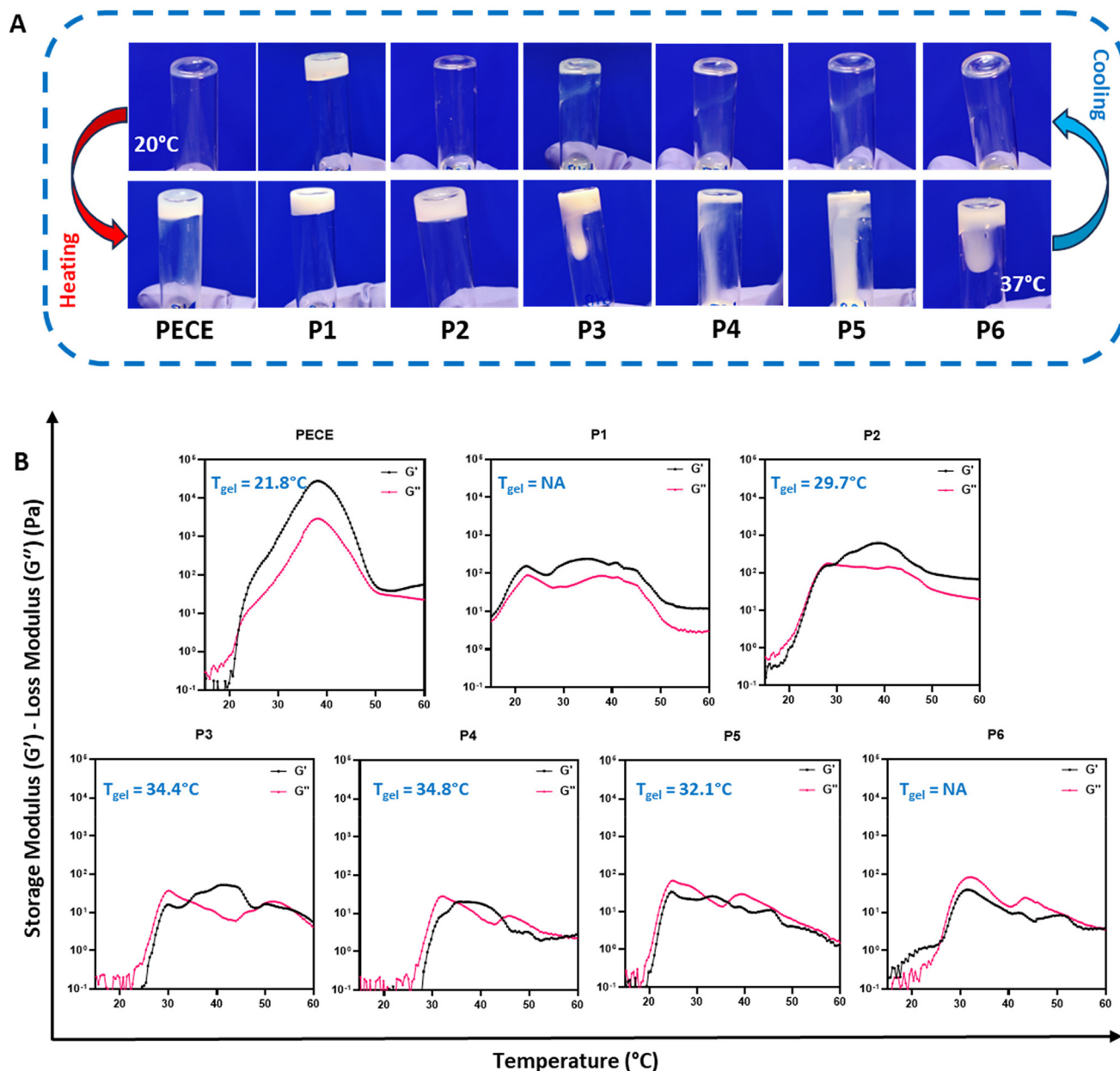
Fig. 1 Thermoresponsive behaviour and rheological properties of polymeric materials. (A) Tube inversion test as a proxy for rheological behaviour of the thermoresponsive polymers (30% w/v) at 20 ^{\circ}\text{C} and 37 ^{\circ}\text{C} . (B) Temperature-dependent changes in storage modulus ( G' ) and loss modulus ( G'' ) for polymeric materials (30% w/v), illustrating their rheological behaviour during the gelation process. ( T_{\text{gel}} = gelation temperature, NA: not applicable).
