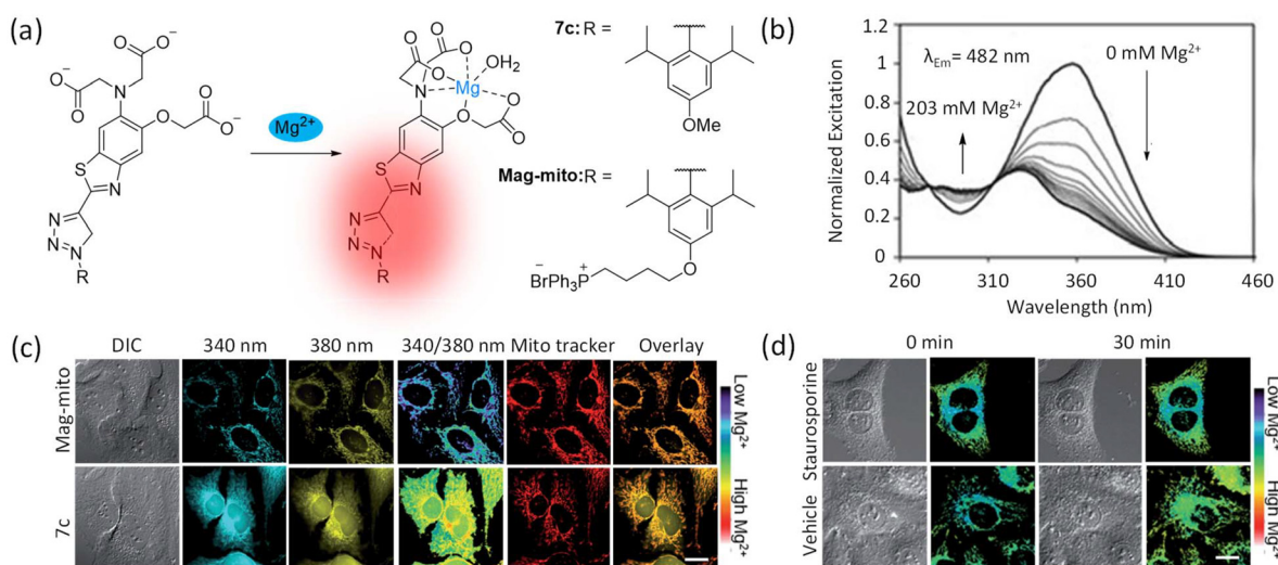
Fig. 9 Imaging and application of the mitochondria-targeted fluorescent probe Mag-mito for the detection of free Mg^{2+} . (a) Response mechanism of triazole-based fluorescent sensor to Mg^{2+} . (b) Fluorescence excitation spectra of probe 7c (2 \mu M) with increasing concentration of MgCl_2 (50 mM PIPES, 100 mM KCl, pH 7.0, 25 ^{\circ} C). (c) Wide-field fluorescence imaging of free Mg^{2+} in the form of acetoxymethyl ester in HeLa cells after treatment with 1 \mu M of Mag-mito targeting mitochondria or non-targeting control 7c. [DIC: phase contrast interferometry image; 340 nm: fluorescence under 340 nm excitation; 380 nm: fluorescence under 380 nm excitation; 340/380 nm: fluorescence ratio under 340/380 nm excitation; Mito Tracker: Mito Tracker green pseudo color in red; overlay of 380 nm channel and mitochondrial staining images]. Zoom bar = 20 \mu m. (d) Wide-field fluorescence imaging of mitochondrial free Mg^{2+} in live HeLa cells treated with 1 \mu M Mag-mito and 1 \mu M apoptosis-inducing staurosporine or vector. DIC images are shown with fluorescence ratiometric controls. Zoom bar = 20 \mu m. Reproduced with permission from ref. 104, Copyright 2015, Royal Society of Chemistry.
