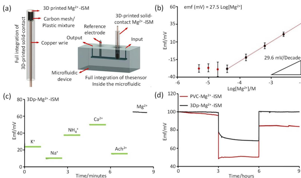
Fig. 8 Design, response characterization and application of 3D printed \text{Mg}^{2+} selective electrodes (3Dp- \text{Mg}^{2+} -ISE). (a) Schematic representation of 3Dp- \text{Mg}^{2+} -ISE integrated into the microfluidic device. (b) The linear response of the 3Dp- \text{Mg}^{2+} -ISE to \text{Mg}^{2+} is observed within a concentration range of 39 \mu\text{M} to 10 mM, showing a slope of 27.5 mV per decade (illustrated error bars are the standard deviation obtained from three separate \text{Mg}^{2+} -ISEs; inset triangle depicts a slope of 29.6 mV per decade). (c) Selectivity analysis of 3Dp- \text{Mg}^{2+} -ISE for different ions (1 mM). (d) The normalized results of the water layer test for PVC- \text{Mg}^{2+} -ISE and 3Dp- \text{Mg}^{2+} -ISE after being immersed in 1 mM \text{Mg}^{2+} solution for 3 hours, then in 1 mM KCl solution for 3 hours, and finally back in 1 mM \text{Mg}^{2+} solution for another 3 hours. Reproduced with permission from ref. 78, Copyright 2023, Royal Society of Chemistry.
