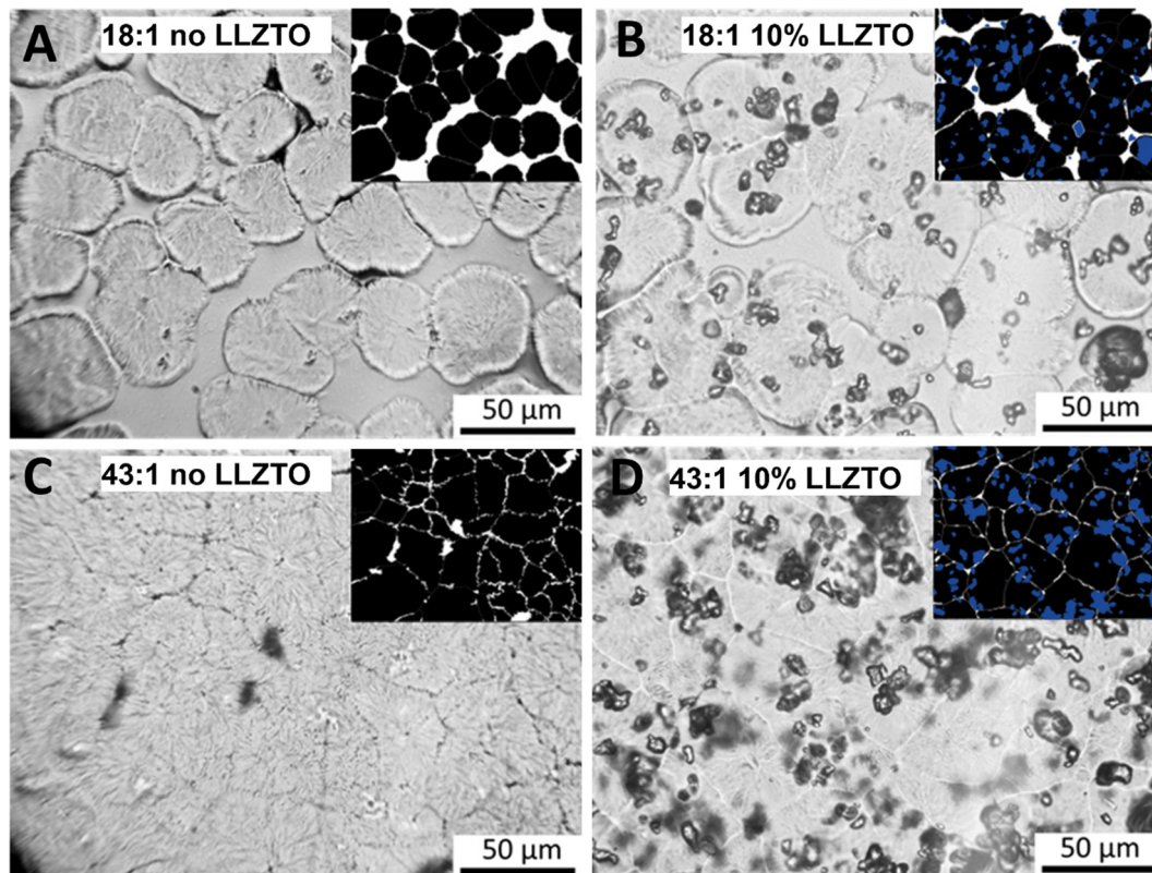
Fig. 2 Optical microscope images of solid-state electrolytes. (A) 18 : 1 no LLZTO, (B) 18 : 1 10% LLZTO, (C) 43 : 1 no LLZTO, and (D) 43 : 1 10% LLZTO. Insets of the same respective fields of view show LLZTO in blue (colors visible in digital version).
