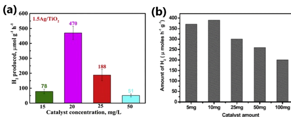
Fig. 25 (a) Photocatalytic hydrogen evolution activity of Ag/ TiO_2 by varying the amount of catalyst. Reproduced with permission from ref. 112. Copyright © 2019, Elsevier Ltd. (b) Variation in photocatalytic H_2 evolution rate with respect to the amount of Ni/\gamma-Al_2O_3/CNT-TiO_2 catalyst. Reproduced with permission from ref. 102. Copyright © 2017, Elsevier Ltd.
