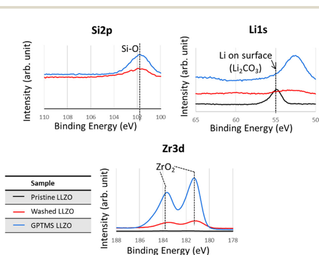
Fig. 5 XPS Si 2p, Li 1s, and Zr 3d spectra of pristine (before functionalization), washed (acid-treated), and GPTMS–LLZO particles. The peak at around 53 eV in Li 1s corresponds to Zr 4s.
