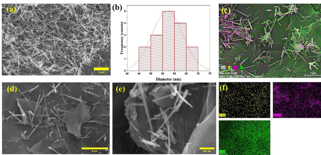
Fig. 1 (a) SEM image of the MnO 2 nano-needles, (b) MnO 2 nano-needles diameter size distribution, (d)–(e) FE-SEM image of the MnO 2 -rGO nanocomposite, and (c) and (f) MnO 2 -rGO nanocomposite elemental mapping.
