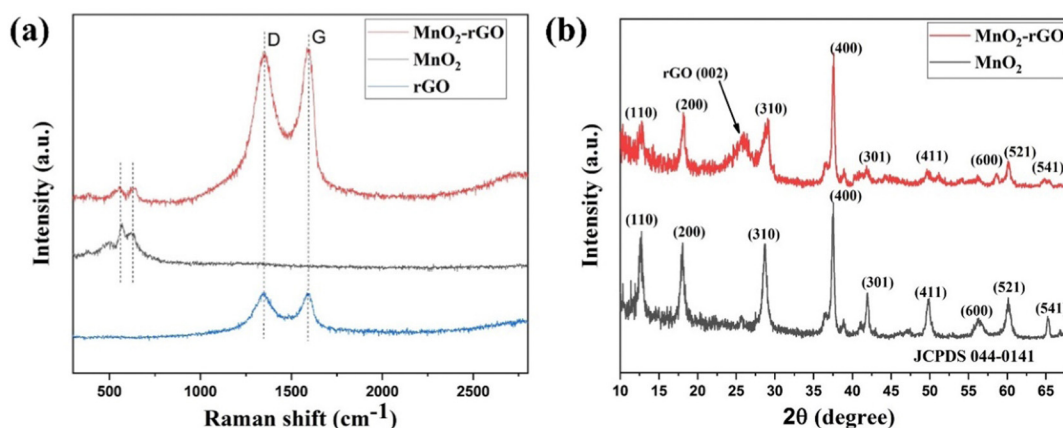
Fig. 2 (a) Raman spectrum of rGO, pure MnO 2 and MnO 2 -rGO, (b) XRD pattern of pure MnO 2 and MnO 2 -rGO.
