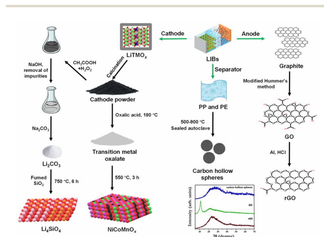
Fig. 2 A schematic illustration of synthesis methodologies adopted for processing LIB's components into functional materials. 37,39,40 The PXRD pattern of synthesised carbon materials reproduced with minor modification from ref. 40 with permission from The Royal Society of Chemistry, copyright 2024.
