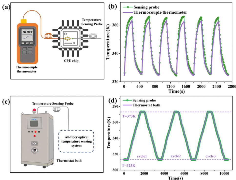
Fig. 10 (a) Schematic diagram of CPU temperature measurement. (b) The real-time temperature variation of CPU. (c) Schematic diagram of thermostat bath temperature measurement. (d) The real-time temperature variation of the thermostat bath.
