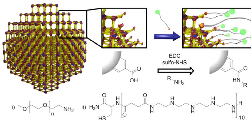
Zimpel and co-workers developed a grafting-to strategy to attach amino-polyethylene glycol (PEG5000, Fig. 9i) and Stp 10-C (a bifunctional polyamide, Fig. 9ii) to the surface of the MOF (Fig. 9). 36 Through a water-based “green” carbodiimide
