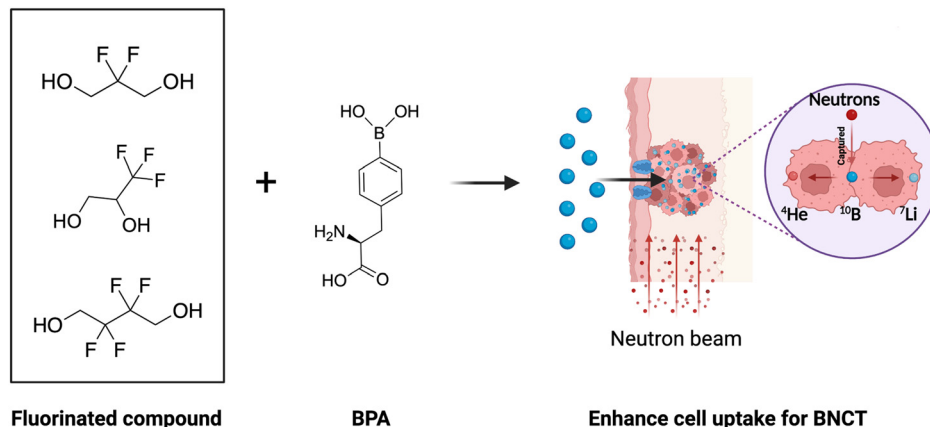
Fig. 1 Schematic illustration of fluorinated BPA derivatives enhancing the ^{10}\text{B} accumulation in tumors in vivo . The figure was created with BioRender.com.
