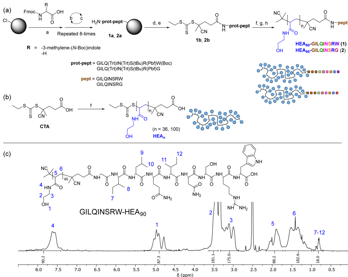
Fig. 1 (a) Synthesis of HEA 90 -GILQINSRW, and HEA 95 -GILQINSRG; (b) synthesis of HEA n as control polymers; (c) 1 H NMR (400 MHz, DMSO-d 6 ) spectra of obtained GILQINSRW-HEA 90 conjugation. Reagents and conditions: (a) DMF, DIPEA, rt; (b) DMF, piperidine, rt; (c) DMF, Fmoc-amino acid, HATU, DIPEA, rt; (d) CTA, HATU, TEA, DMF, rt; (e) DCM/TFE 8 : 2 v/v, rt; (f) N -hydroxyethyl acrylamide, V501, DMF, 70 °C; (g) AIBN, DMF, 80 °C; (h) 0.1 N HCl in hexafluoro-2-propanol (HFIP), rt.
