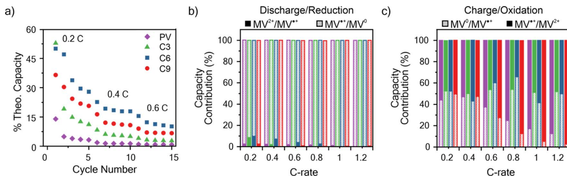
Fig. 6 (a) Discharge capacity summary for the polymers studied at varying C-rates. (b) The percent of total discharge (reduction) capacity from the MV 2+ /MV + and MV + /MV 0 redox couples at varying C-rates. (c) The percent of total charge (oxidation) capacity from the MV 0 /MV + and MV + /MV 2+ redox couples at varying C-rates. The data is taken from the first galvanostatic charge–discharge cycle at each C-rate in Fig. S31.† The colors corresponding to each polymer in panel (a) are applicable to panels (b) and (c). The working electrodes were tested in a half cell against lithium metal. The working electrode was polymer thin film on ITO-coated glass and 0.5 M LiCl in GBL on filter paper as the supporting electrolyte and separator, respectively.
