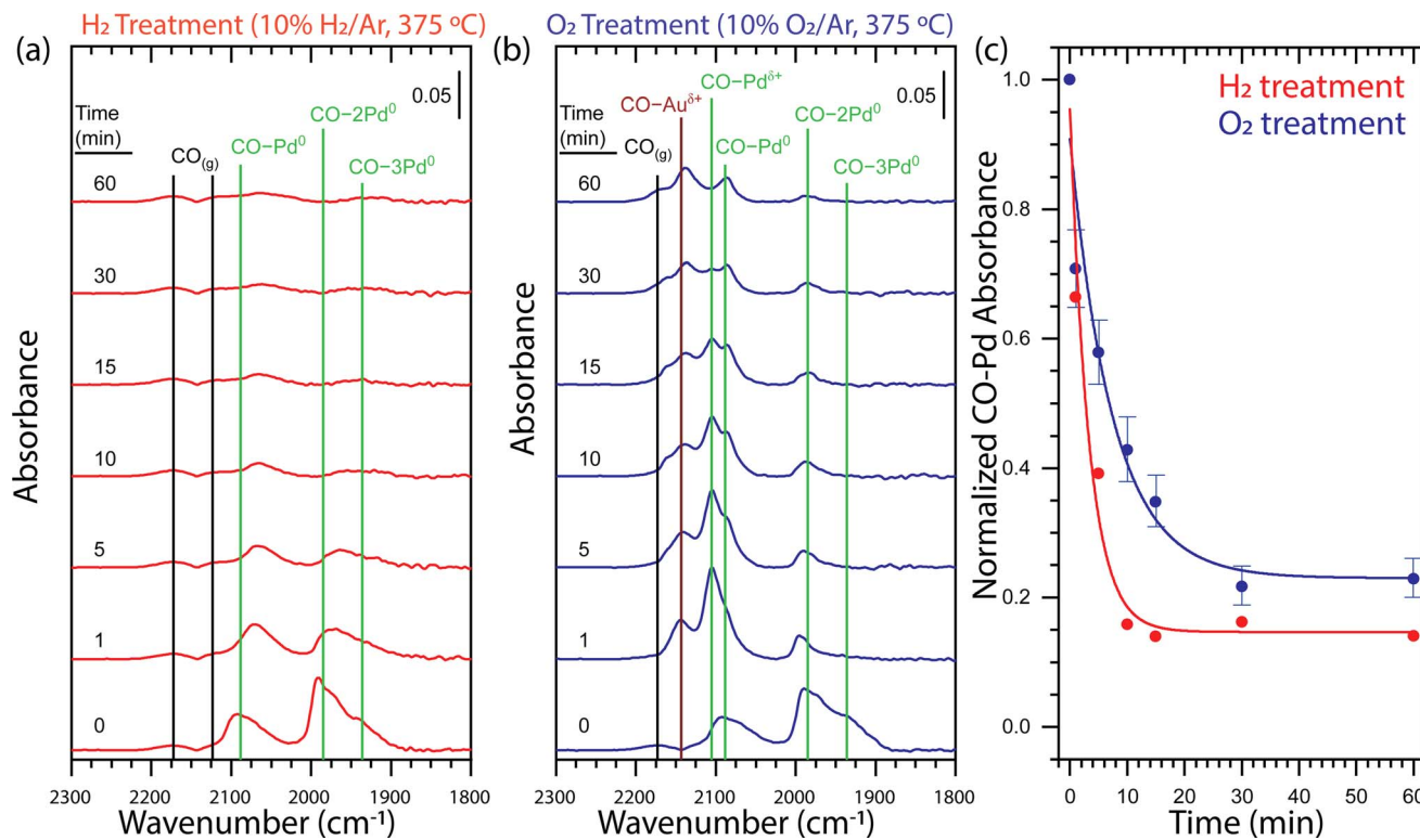
Fig. 3 Time-dependent DRIFT spectra for (a) \text{H}_2 and (b) \text{O}_2 treatments of core-shell Au-Pd/SiO 2 probed by CO adsorption demonstrate that the dissolution of Pd from the surface strongly depends on the gas environment. (c) Integrated CO-Pd bands of ex situ time-dependent DRIFT spectra for \text{H}_2 (red) and \text{O}_2 (blue) treatments of core-shell Au-Pd/SiO 2 normalized at t = 0 demonstrate that the \text{H}_2 treatment causes faster Pd dissolution and yields a lower Pd surface concentration. The guidelines through the \text{H}_2 and \text{O}_2 treatment integrated data are fitted with an exponential decay function. The error bars associated to the \text{O}_2 data points originate from the errors in the deconvolution of the CO-Pd peaks, as explained in Fig. S6.† The vibrational feature assignments are tabulated in Table S1† and additional evidence for the assignments are provided in Fig. S5.† Each spectrum panel denotes a 0.05 absorbance intensity legend. \text{H}_2 pretreatment: 5% \text{H}_2 in Ar, 250 °C, 45 min; \text{H}_2 treatment: 10% \text{H}_2 in Ar, 375 °C; \text{O}_2 treatment: 10% \text{O}_2 in Ar, 375 °C; CO adsorption conditions: 0.1% CO in Ar, 25 °C.
