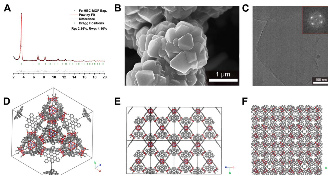
Fig. 2 Experimental and Pawley-refined powder X-ray diffraction pattern of the Fe-HBC-MOF (A), SEM image of the octahedral intergrown crystallites with sizes up to 600–900 nm (B), TEM image of MOF crystallites. Inset: FFT taken for the crystallite examined (C) and display of the simulated structure of Fe-HBC-MOF with a view on the open supertetrahedron (D), view on the tetrahedral arrangement of the c -HBC ligands in the unit cell (E) and view along the c -axis showing the pore system (F).
