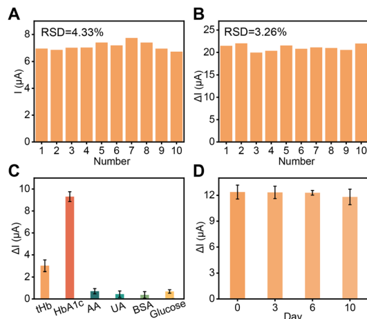
Fig. 4 (A) SWV responses of ten independent CRISPR-amplified aptasensors for HbA1c detection under the same conditions. (B) \Delta I of ten independent CRISPR-amplified aptasensors for 100 μg mL -1 HbA1c detection. (C) \Delta I of this aptasensor for the detection of tHb, HbA1c, AA, UA, BSA and glucose. (D) The storage stability of this aptasensor. The error bars represent the standard deviation of at least three independent measurements.
