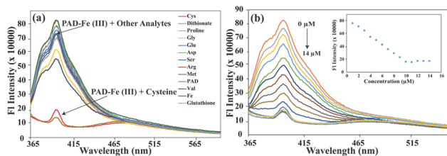
Fig. 3 (a) Emission spectra of the probe PAD C Fe(III) ensemble (5 μM) upon addition of different amino acids and bio-thiols (50 μM) in HEPES buffer solution (1 mM, pH = 7.4); (b) emission spectra of the PAD C Fe(III) ensemble with different concentrations of cysteine [inset: a linear correlation between the emission intensity at 398 nm and the concentration of Cys. \lambda_{\text{ex}} = 350 nm].
