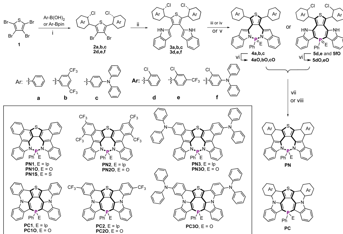
Scheme 1 Synthesis of new P-PAMs with isomeric structures. (i) Pd(PPh 3 ) 4 , base, solvent, \Delta . (ii) Pd(OAc) 2 , Ruphos, K 3 PO 4 , solvent, \Delta . (iii) PhPCl 2 , DBU, acetonitrile. (iv) PPhCl 2 (1.3 eqv.), TMSOTf (2.6 eqv.), CH 3 CN, -30^\circ\text{C} \rightarrow 70^\circ\text{C} . (v) PhP(O)H(OH), DMAP, -30^\circ\text{C} \rightarrow 70^\circ\text{C} . (vi) H 2 O 2 (excess), r.t. in DCM. (vii) DDQ, 365 nm LED, dry toluene, r.t. (viii) CuI, K 3 PO 4 , DMEDA, DMF, 140^\circ\text{C} .
